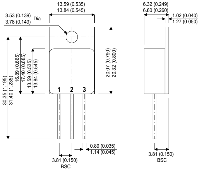
TO-254 Package.
